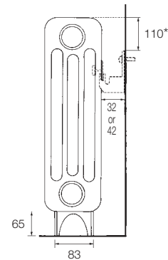
Cast Iron Floor Bracket and Clamp
